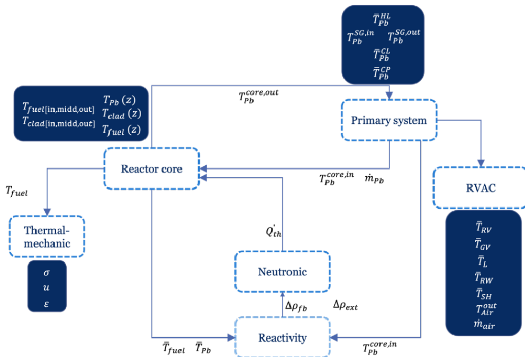
Figure 7. Main modules and feedback in BELLA code.
