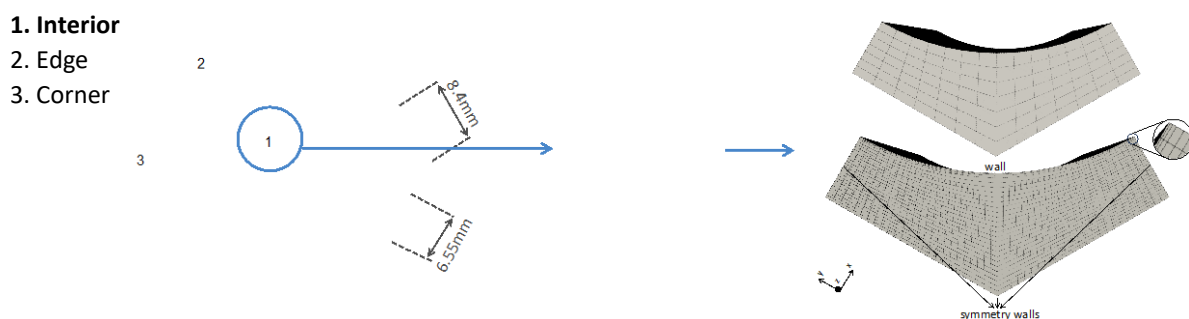
Figure 11. Sketch of the IPS fuel hexagonal sub-assembly and the zoom on the interior sub-channel with the considered computational domain highlighted in blue (left and center). On the right, the coarser (top) and the finer (bottom) meshes of the coolant domain adopted for the grid independence study are shown (Table 9).
