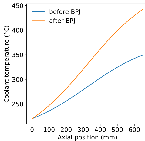
Figure 28. Coolant temperature along the length of the IPS sub-channel, before and after the BPJ transient scenario considered.
