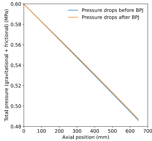
Figure 25. Total LBE pressure drops (gravitational and frictional) evaluated via OpenFOAM (same result from both Huang and Kays correlations for the turbulent Prandtl number).
