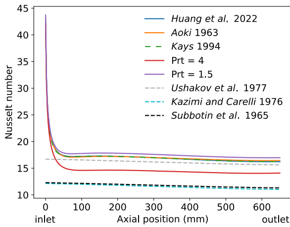
Figure 15. Comparison along the length of the sub-channel of the Nusselt number evaluated using the selected Pr_t models (by Aoki 1963, Kays 1994 and Huang 2022) and using constant Pr_t equal to 1.5 and 4, under MYRRHA normal operating conditions. The Nusselt numbers predicted by the empirical correlations for LBE reported in Table 5 are additionally reported (dashed lines).
