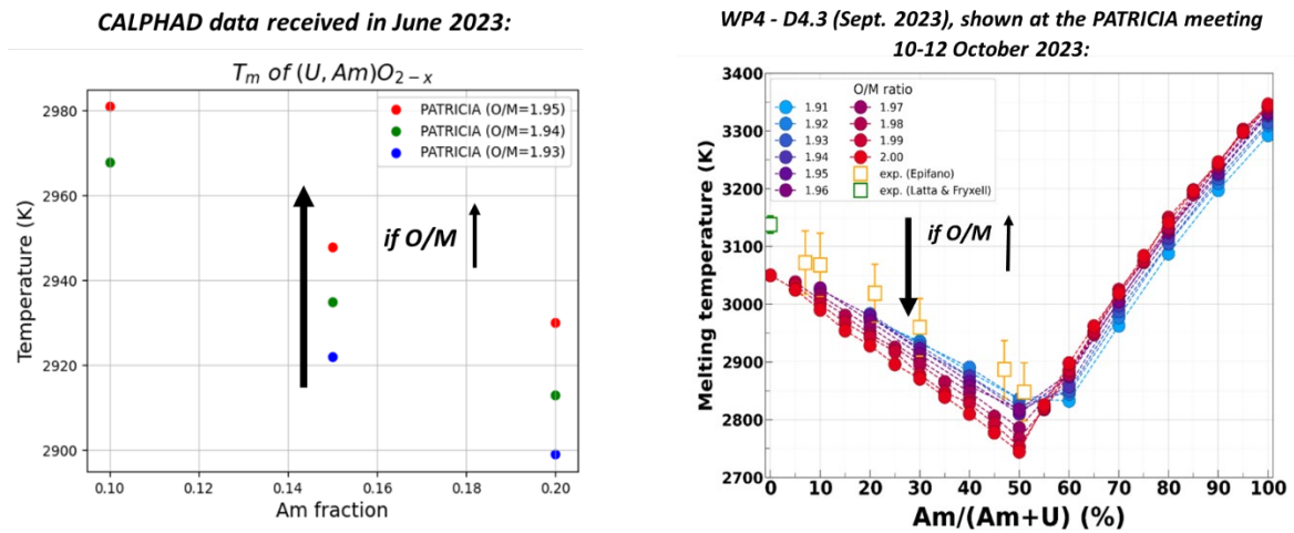
Figure 8: Behaviour of the melting temperature of (U,Am)O_{2-x} as a function of the Am content, for different O/M values, as predicted by CALPHAD modelling (left) or atomic-scale calculations (right).
