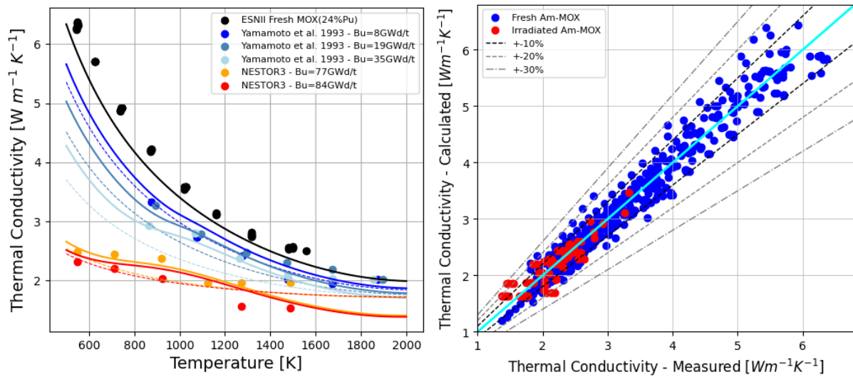
Figure 3: Left: Comparison of the novel model proposed for the thermal conductivity of (U,Pu,Am)O 2-x (full lines) and of the model already published in [15] (dashed lines), as a function of temperature, in comparison with experimental data on irradiated fuels. Right: Comparison of the model predictions with the data considered.
