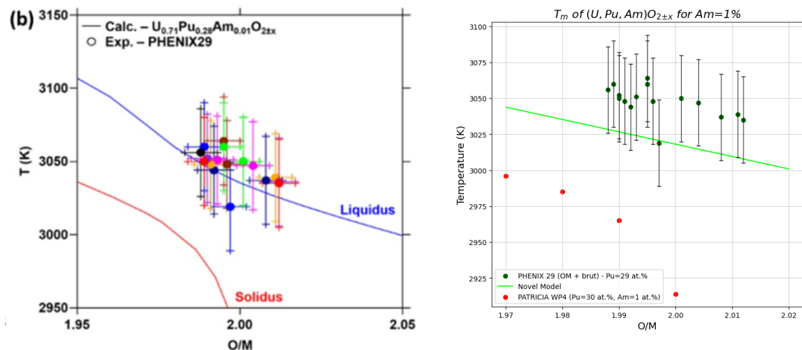
Figure 9: Experimental data on the melting temperature (solidus / liquidus) of Phénix U-Pu-Am-O fuel, compared to part of the phase diagram from CALPHAD obtained during the former INSPYRE Project (left), while to the novel model proposed (Section 2.2) and to novel CALPHAD data from PATRICIA WP4 for similar fuel composition (right).
